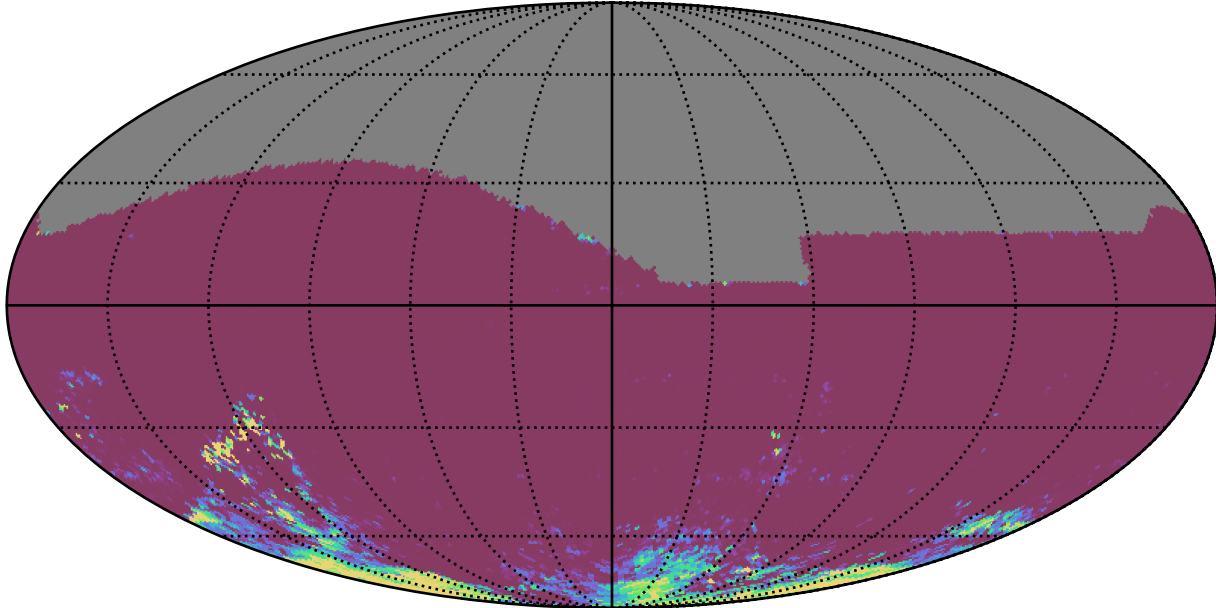
ddf_acor_sf25_lsf40_lsr20_v3.4_10yrs All sky ri bands: 75th Percentile Intranight Timespan
