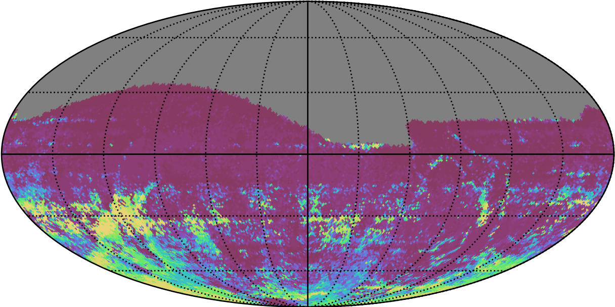
ddf_acor_sf25_lsf40_lsr20_v3.4_10yrs All sky r band: 75th Percentile Intranight Timespan
