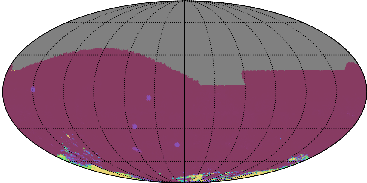
ddf_acor_sf25_lsf40_lsr20_v3.4_10yrs All sky iz bands: 75th Percentile Intranight Timespan
