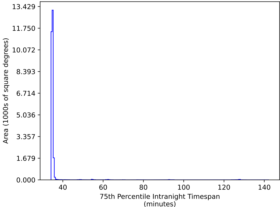
ddf_acor_sf25_lsf40_lsr20_v3.4_10yrs All sky iz bands: 75th Percentile Intranight Timespan
