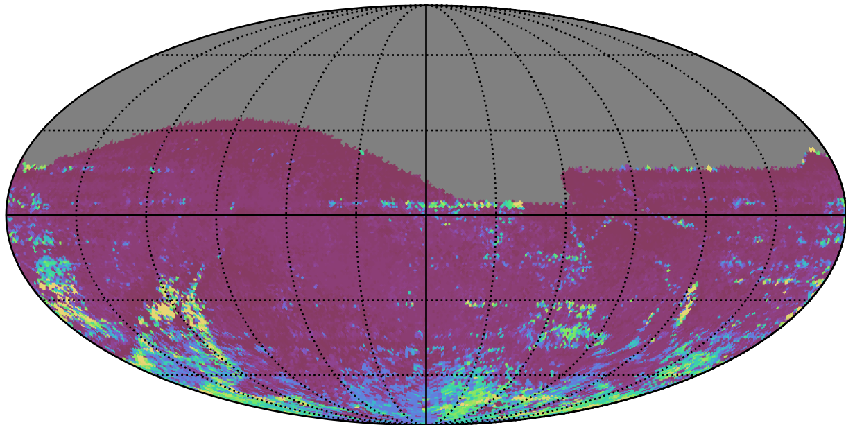
ddf_acor_sf25_lsf40_lsr20_v3.4_10yrs All sky i band: 75th Percentile Intranight Timespan
