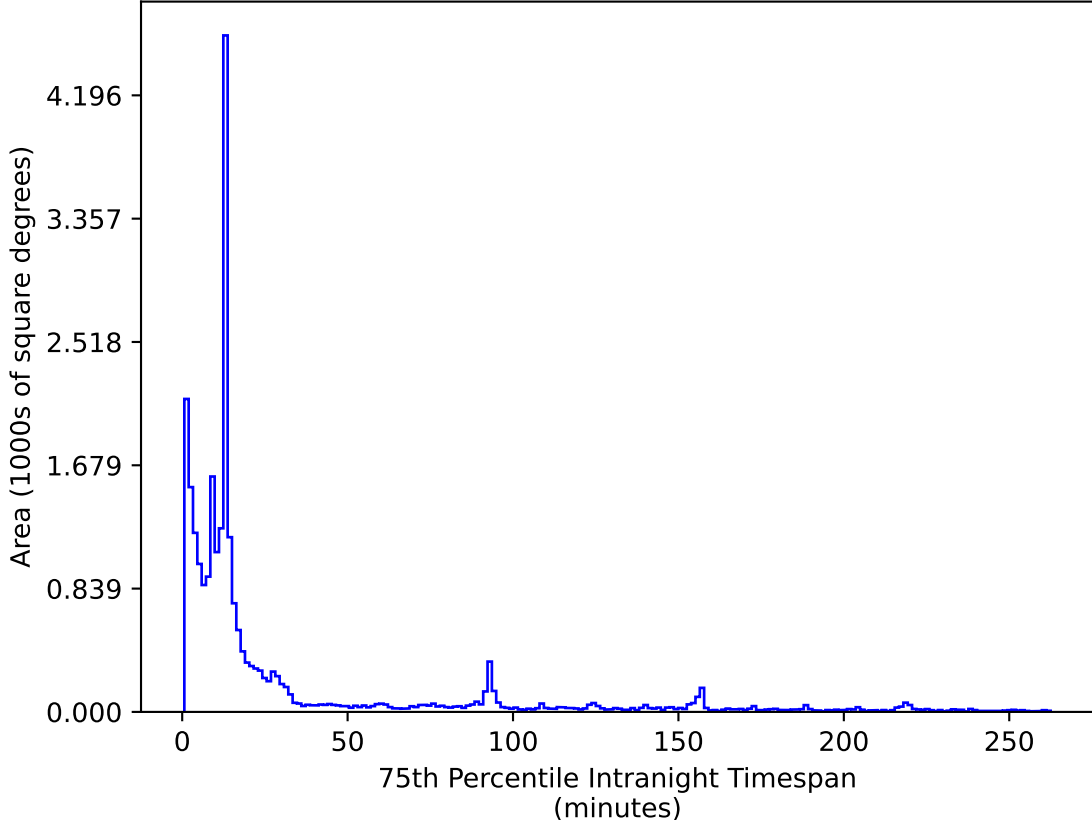
ddf_acor_sf25_lsf40_lsr20_v3.4_10yrs All sky i band: 75th Percentile Intranight Timespan
