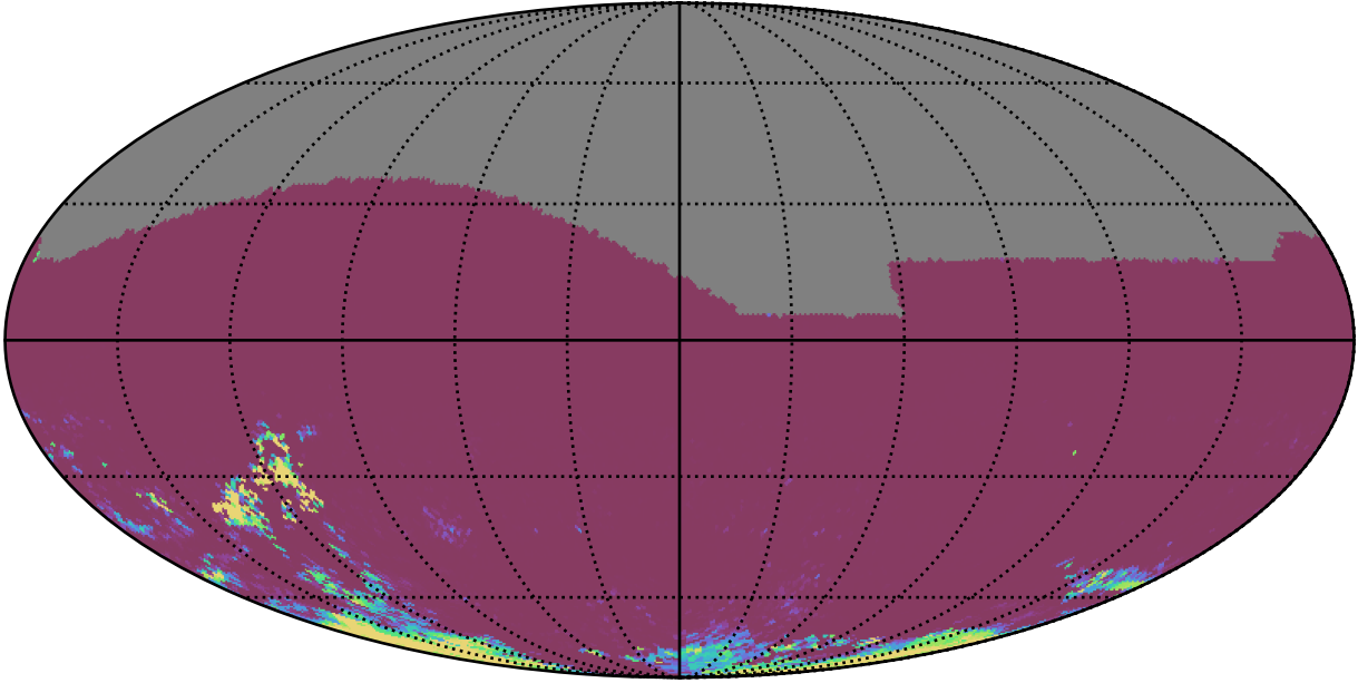
ddf_acor_sf25_lsf40_lsr20_v3.4_10yrs All sky gr bands: 75th Percentile Intranight Timespan
