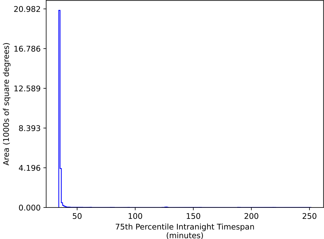
ddf_acor_sf25_lsf40_lsr20_v3.4_10yrs All sky gr bands: 75th Percentile Intranight Timespan
