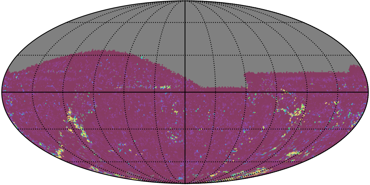
ddf_acor_sf25_lsf40_lsr20_v3.4_10yrs All sky g band: 75th Percentile Intranight Timespan
