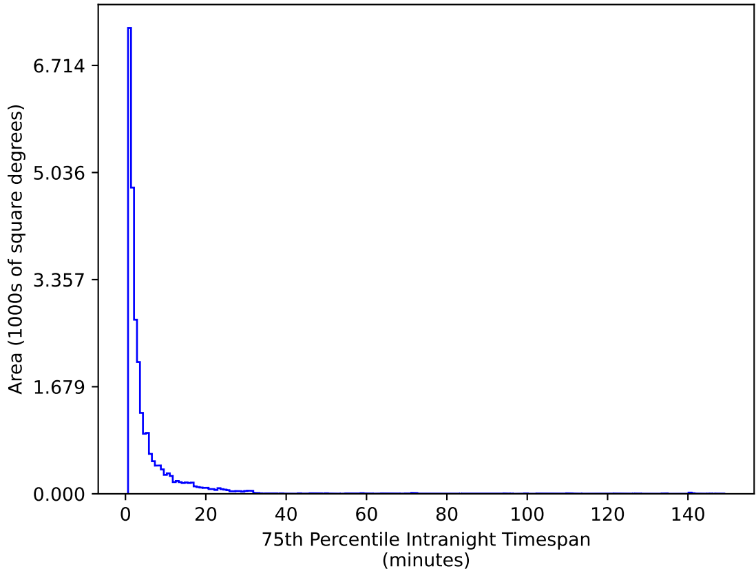
ddf_acor_sf25_lsf40_lsr20_v3.4_10yrs All sky g band: 75th Percentile Intranight Timespan
