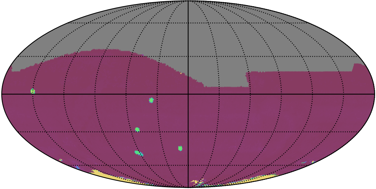
ddf_acor_sf25_lsf40_lsr20_v3.4_10yrs All sky all bands: 75th Percentile Intranight Timespan
