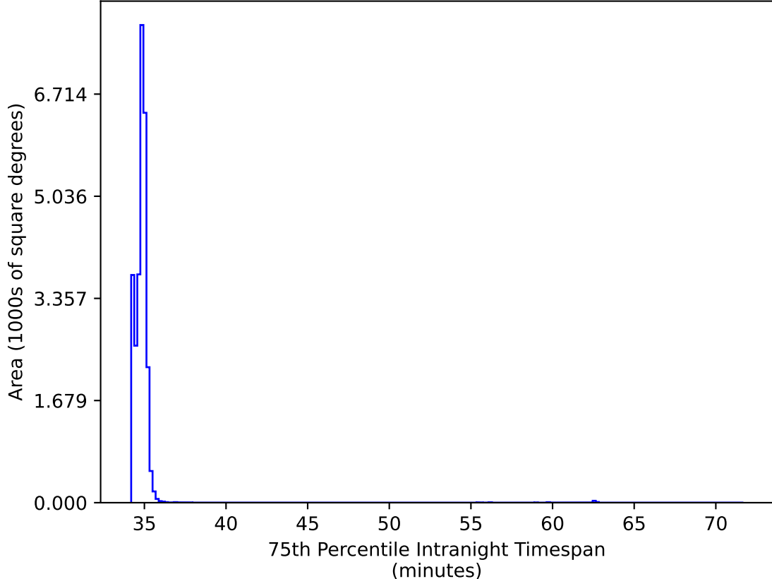
ddf_acor_sf25_lsf40_lsr20_v3.4_10yrs All sky all bands: 75th Percentile Intranight Timespan
