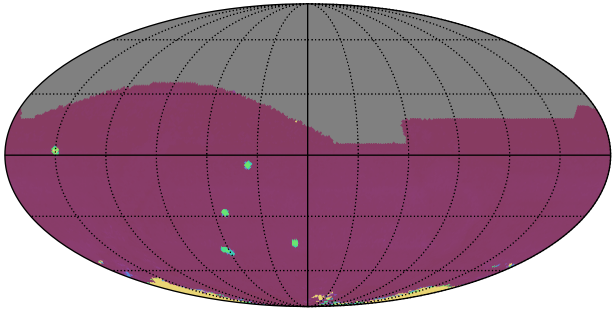
ddf_acor_sf25_lsf40_lsr20_v3.4_10yrs All sky: 75th Percentile Intranight Timespan
