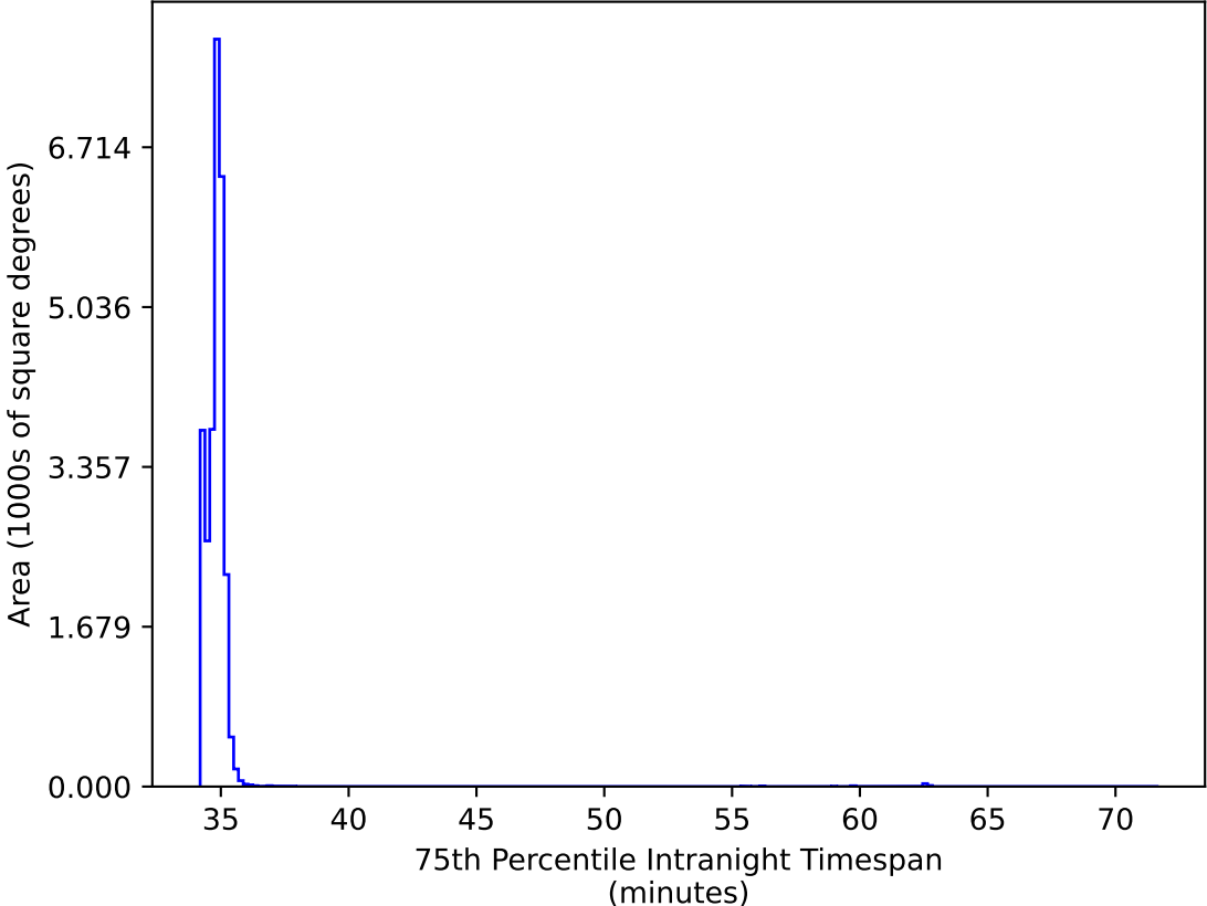
ddf_acor_sf25_lsf40_lsr20_v3.4_10yrs All sky: 75th Percentile Intranight Timespan
