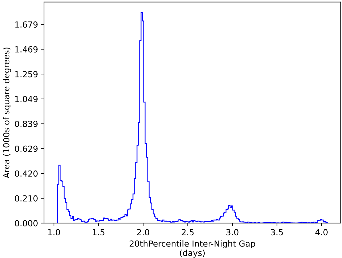
ddf_acor_sf25_lsf40_lsr20_v3.4_10yrs WFD y band: 20thPercentile Inter-Night Gap
