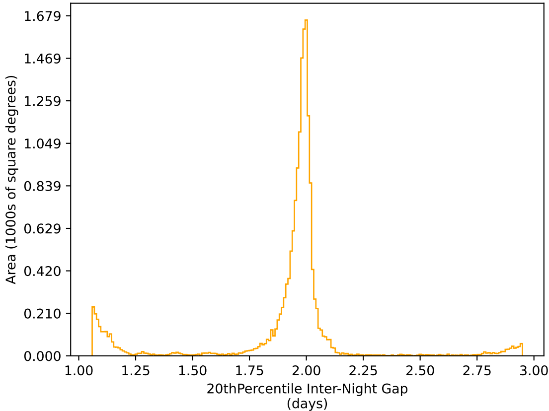
ddf_acor_sf25_lsf40_lsr20_v3.4_10yrs WFD r band: 20thPercentile Inter-Night Gap
