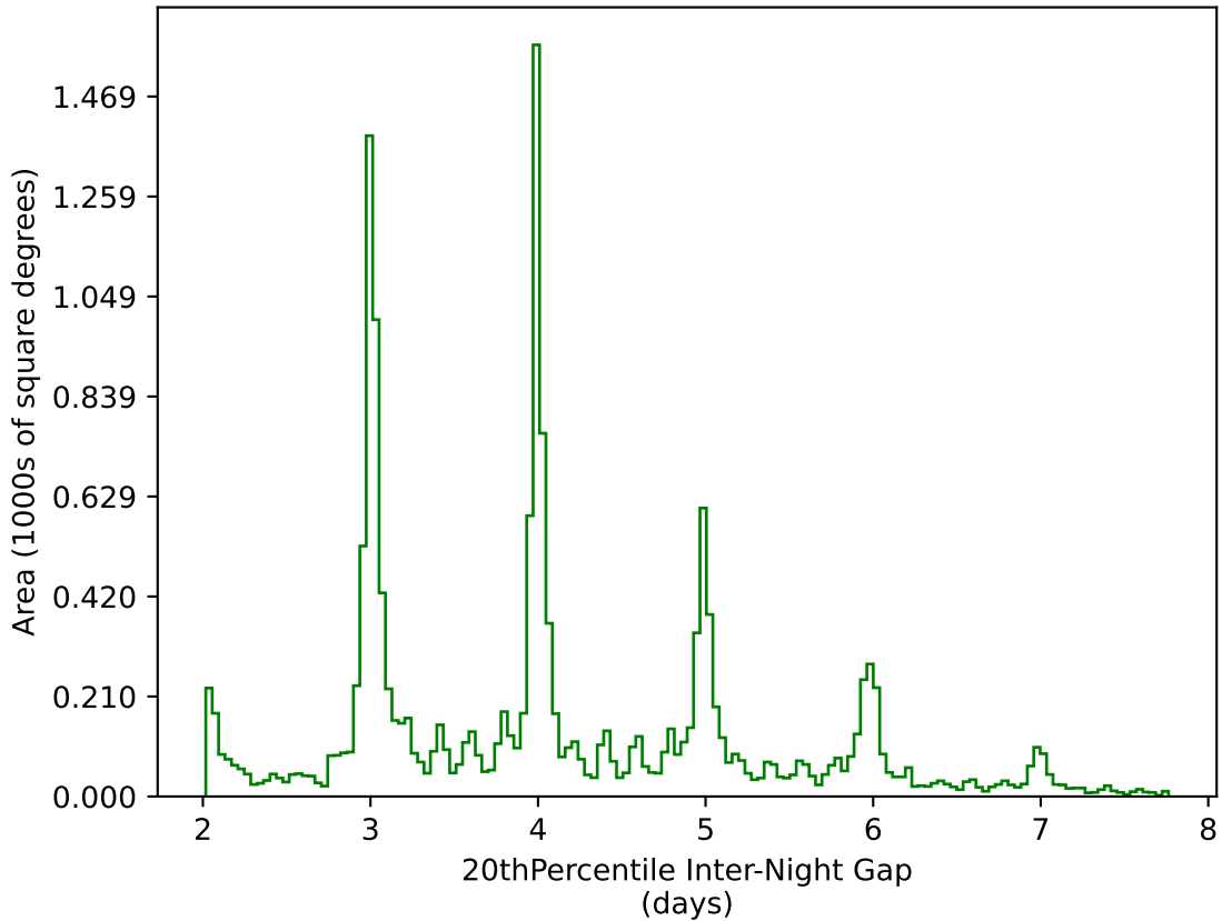
ddf_acor_sf25_lsf40_lsr20_v3.4_10yrs WFD g band: 20thPercentile Inter-Night Gap
