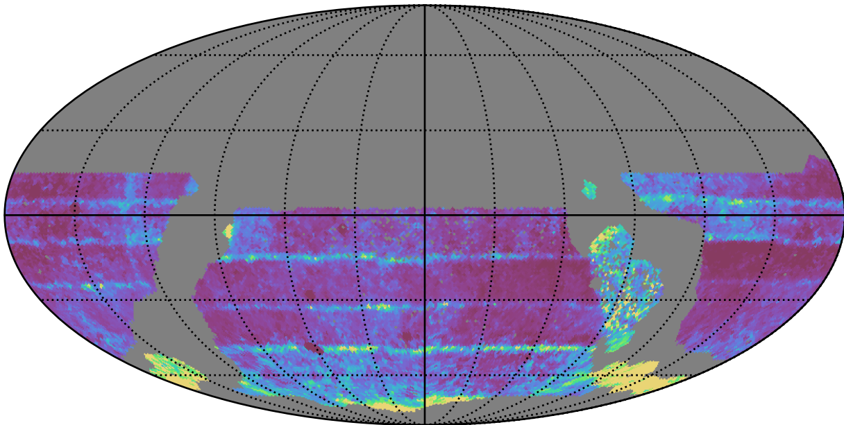
ddf_acor_sf25_lsf40_lsr20_v3.4_10yrs WFD all bands: 20thPercentile Inter-Night Gap
