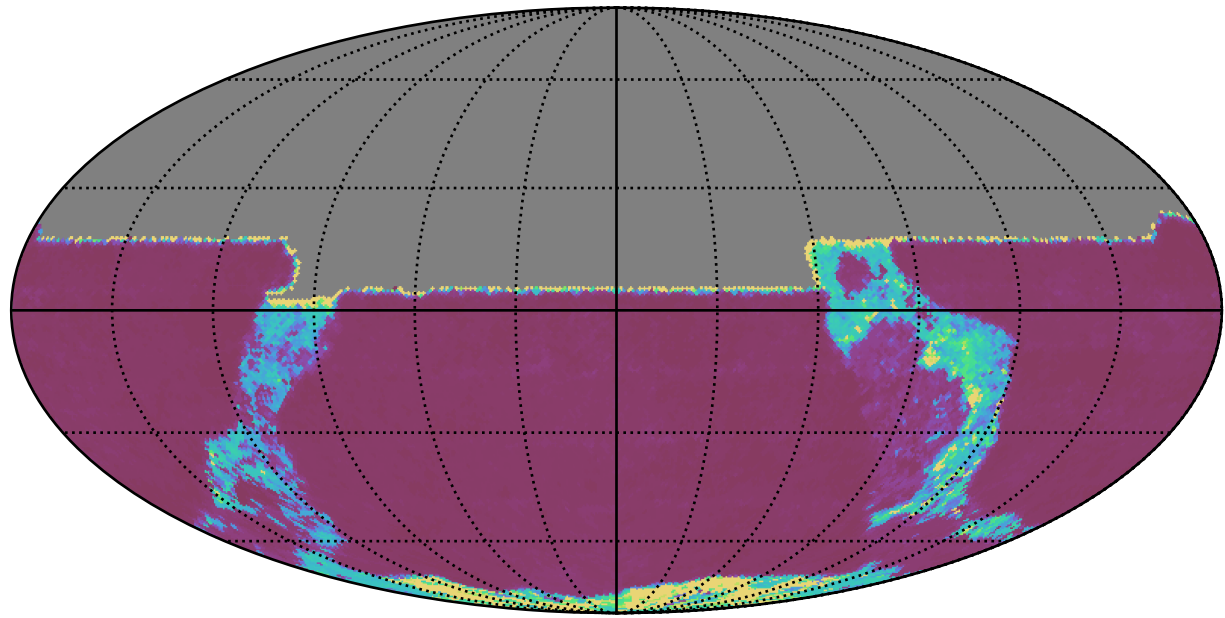
ddf_acor_sf25_lsf40_lsr20_v3.4_10yrs All sky y band: 20thPercentile Inter-Night Gap
