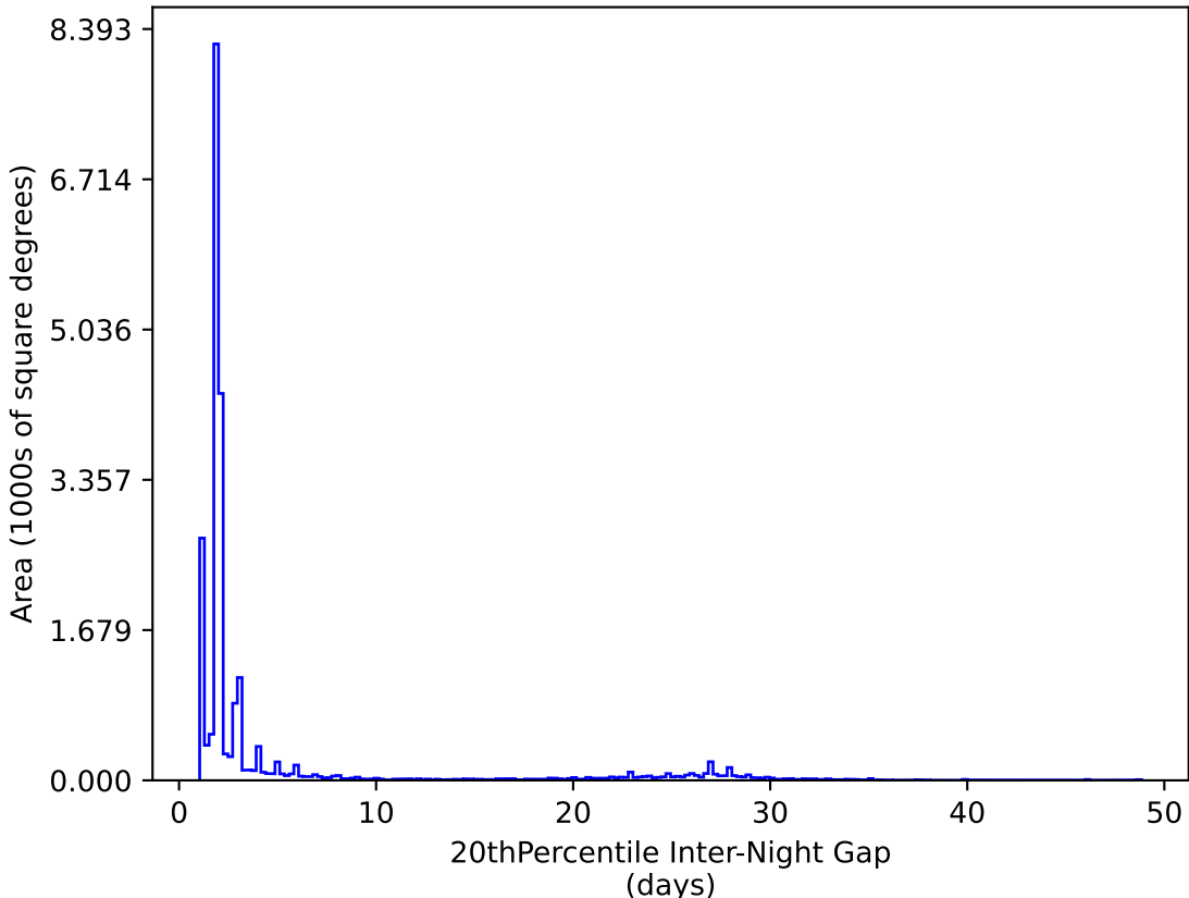
ddf_acor_sf25_lsf40_lsr20_v3.4_10yrs All sky y band: 20thPercentile Inter-Night Gap
