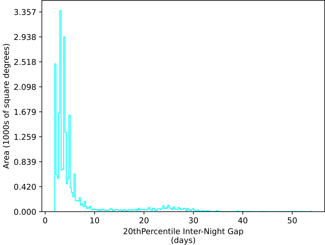
ddf_acor_sf25_lsf40_lsr20_v3.4_10yrs All sky u band: 20thPercentile Inter-Night Gap
