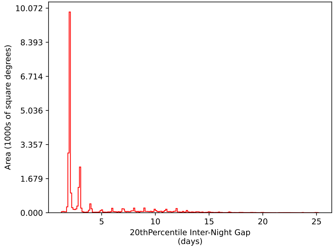
ddf_acor_sf25_lsf40_lsr20_v3.4_10yrs All sky i band: 20thPercentile Inter-Night Gap
