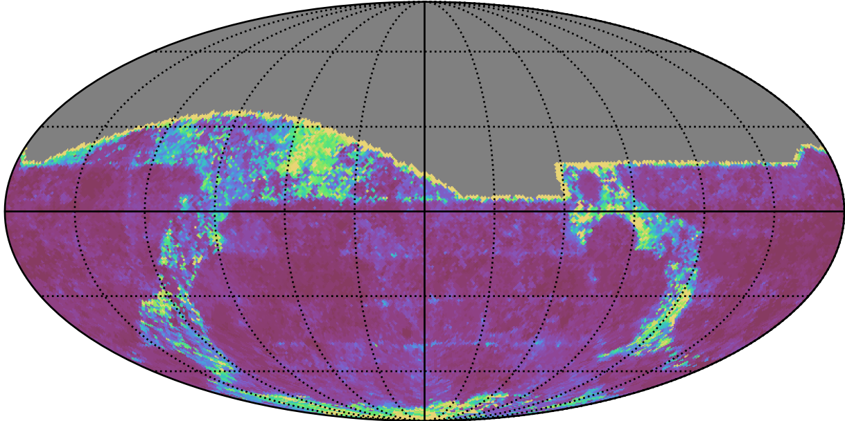
ddf_acor_sf25_lsf40_lsr20_v3.4_10yrs All sky g band: 20thPercentile Inter-Night Gap
