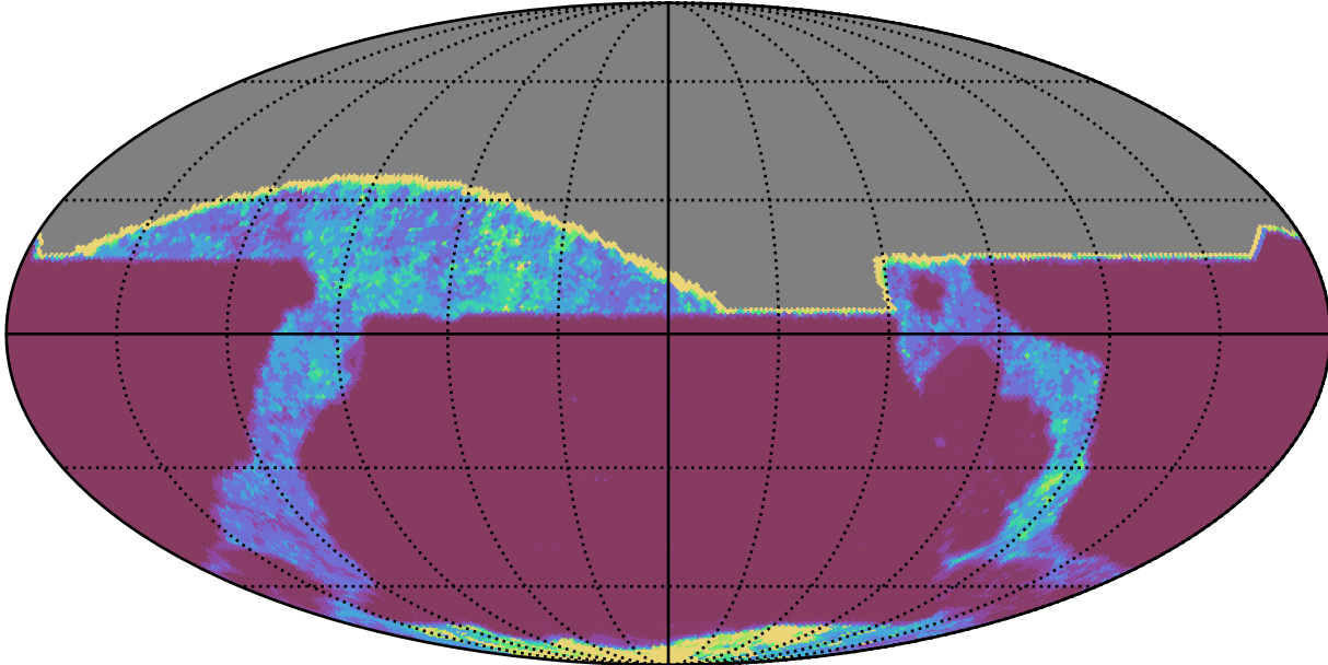
ddf_acor_sf25_lsf40_lsr20_v3.4_10yrs All sky all bands: 20thPercentile Inter-Night Gap
