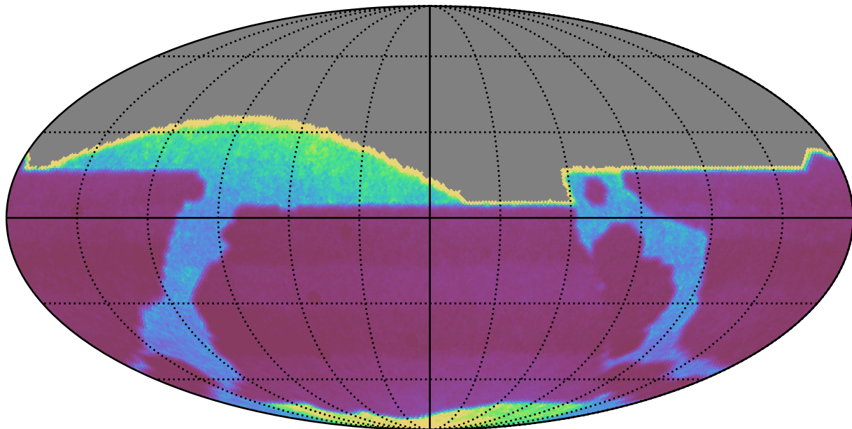
ddf_acor_sf25_lsf40_lsr20_v3.4_10yrs : properMotion
