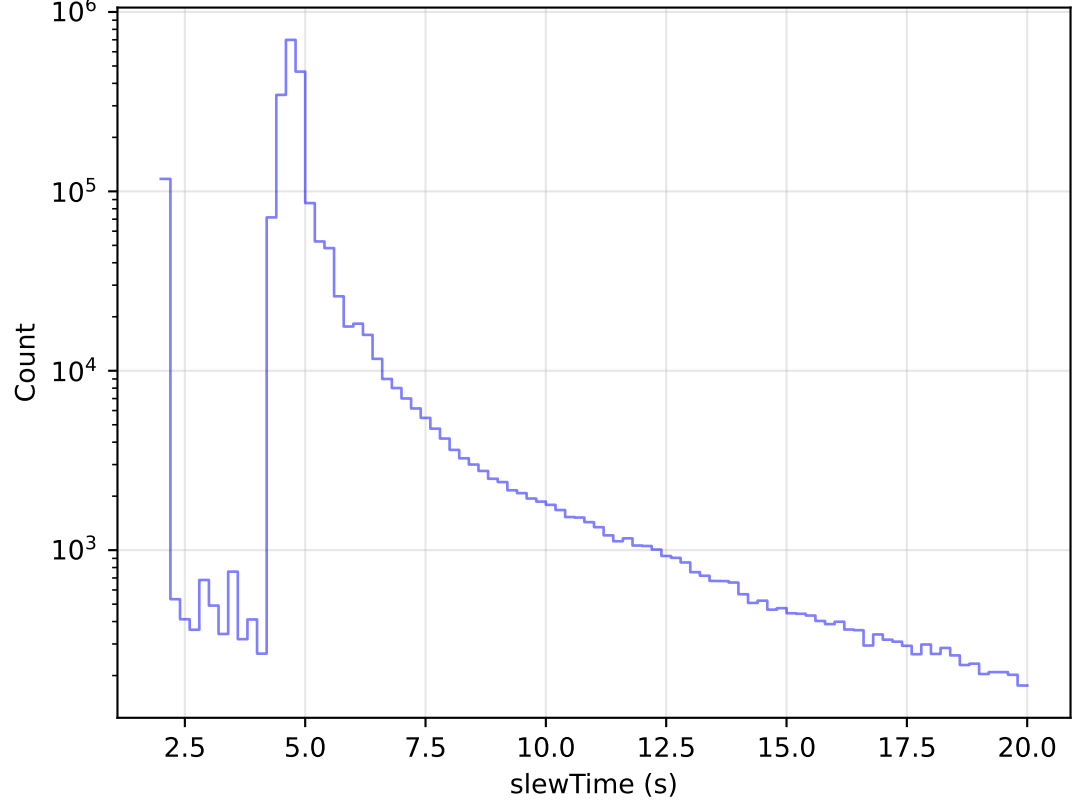
ddf_acor_sf25_Isf40_Isr20_v3.4_10yrs All visits: Zoom Slew Time Histogram
