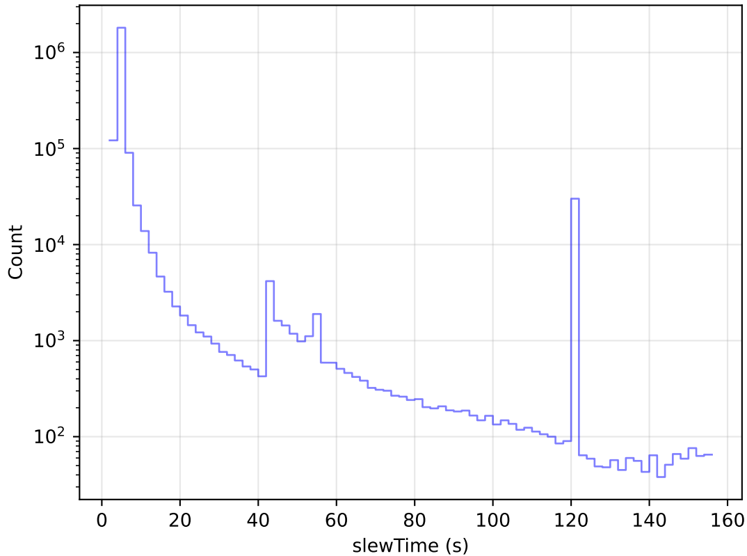
ddf_acor_sf25_lsf40_lsr20_v3.4_10yrs All visits: Slew Time Histogram
