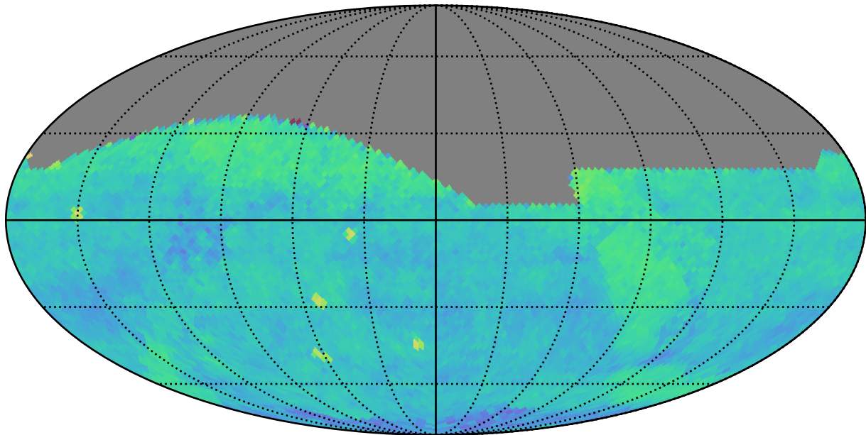
ddf_acor_sf25_lsf40_lsr20_v3.4_10yrs (g or r or i): PairFraction
