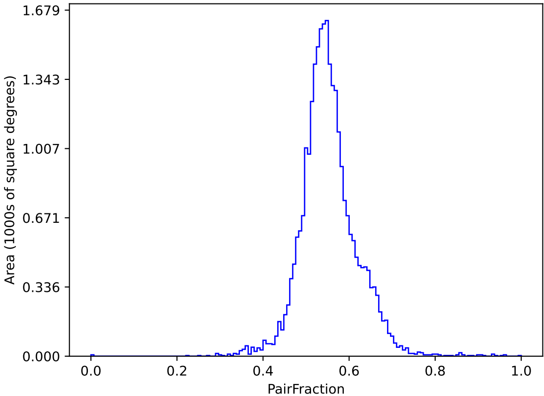
ddf_acor_sf25_lsf40_lsr20_v3.4_10yrs (g or r or i): PairFraction
