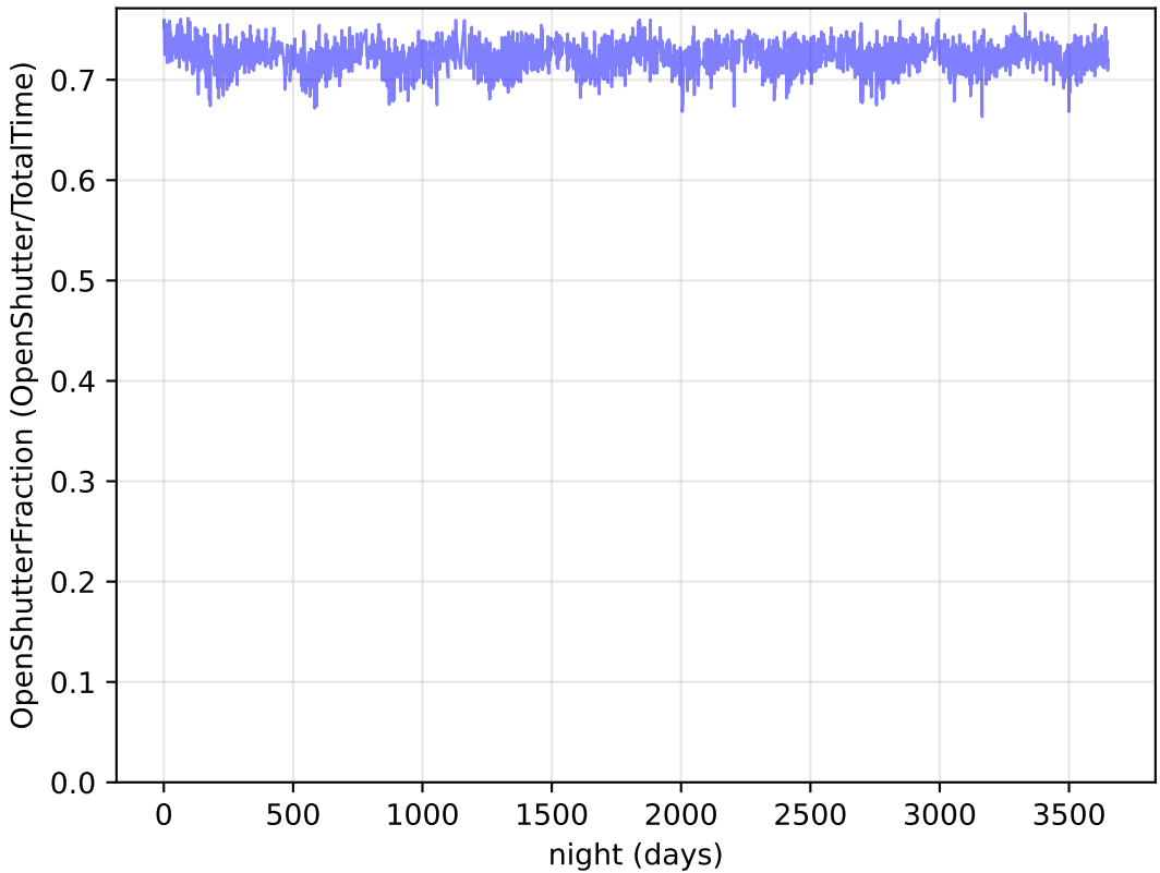
ddf_acor_sf25_lsf40_lsr20_v3.4_10yrs : OpenShutterFraction
