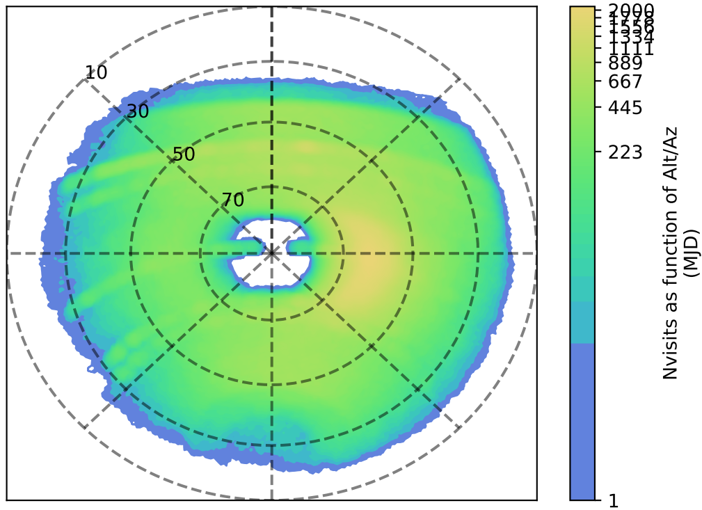
ddf_acor_sf25_lsf40_lsr20_v3.4_10yrs y: Nvisits as function of Alt/Az
