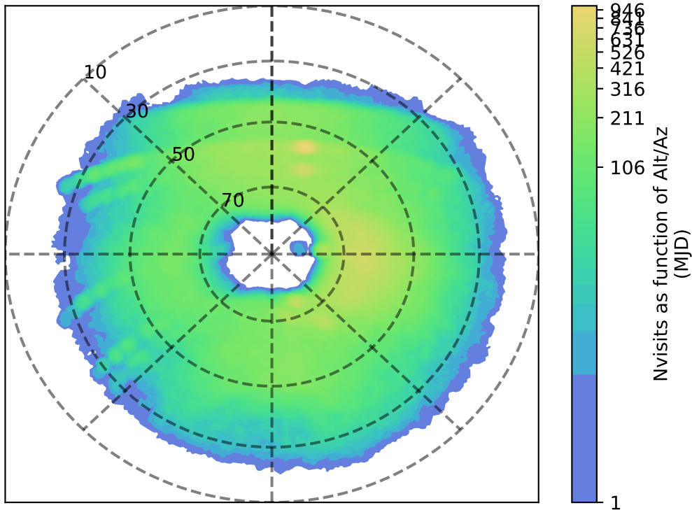
ddf_acor_sf25_lsf40_lsr20_v3.4_10yrs u: Nvisits as function of Alt/Az
