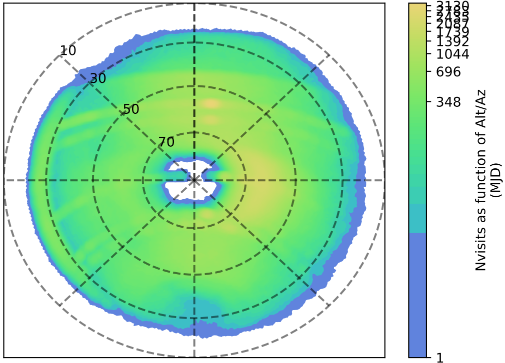
ddf_acor_sf25_lsf40_lsr20_v3.4_10yrs r: Nvisits as function of Alt/Az
