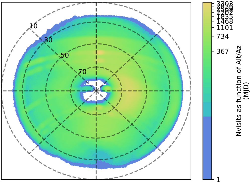
ddf_acor_sf25_lsf40_lsr20_v3.4_10yrs i: Nvisits as function of Alt/Az
