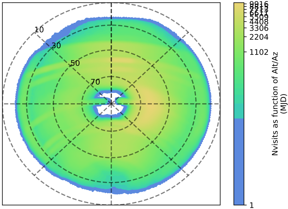
ddf_acor_sf25_lsf40_lsr20_v3.4_10yrs : Nvisits as function of Alt/Az
