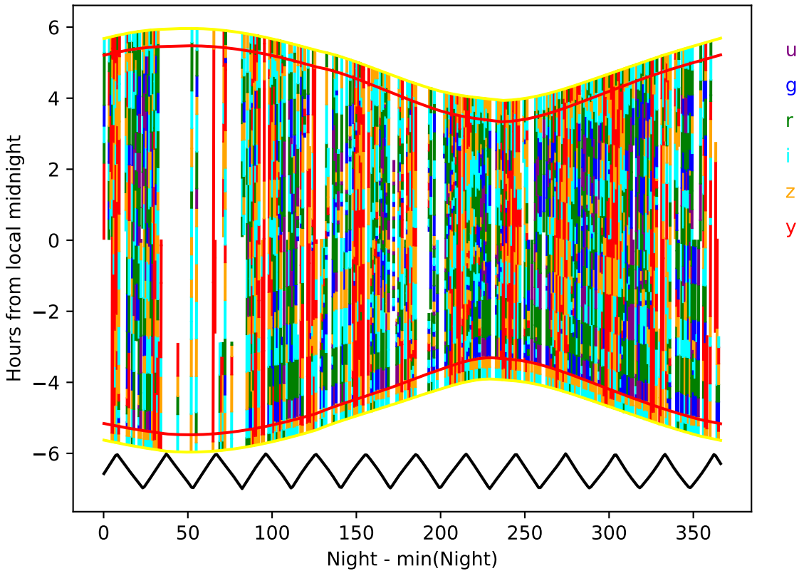
ddf_acor_sf25_lsf40_lsr20_v3.4_10yrs year 3-4: Hourglass
