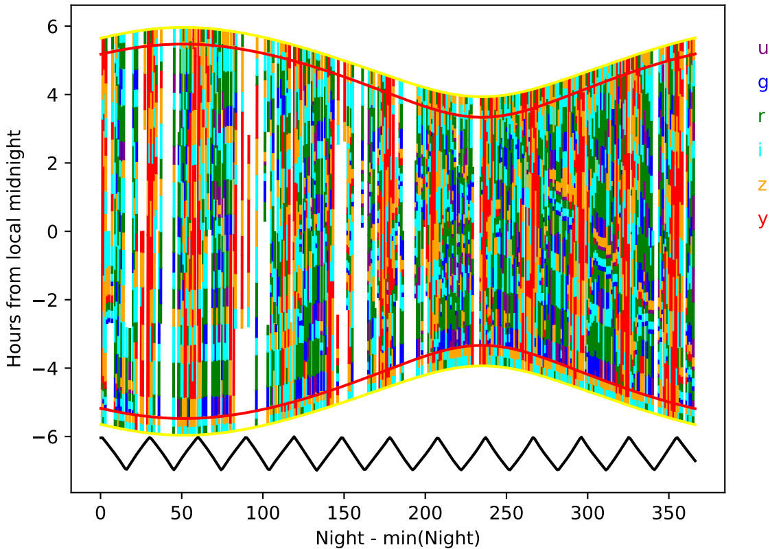
ddf_acor_sf25_lsf40_lsr20_v3.4_10yrs year 1-2: Hourglass
