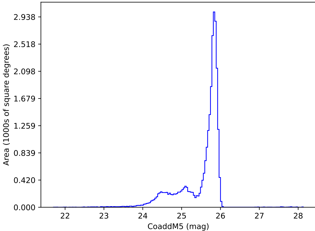
ddf_acor_sf25_lsf40_lsr20_v3.4_10yrs z: CoaddM5
