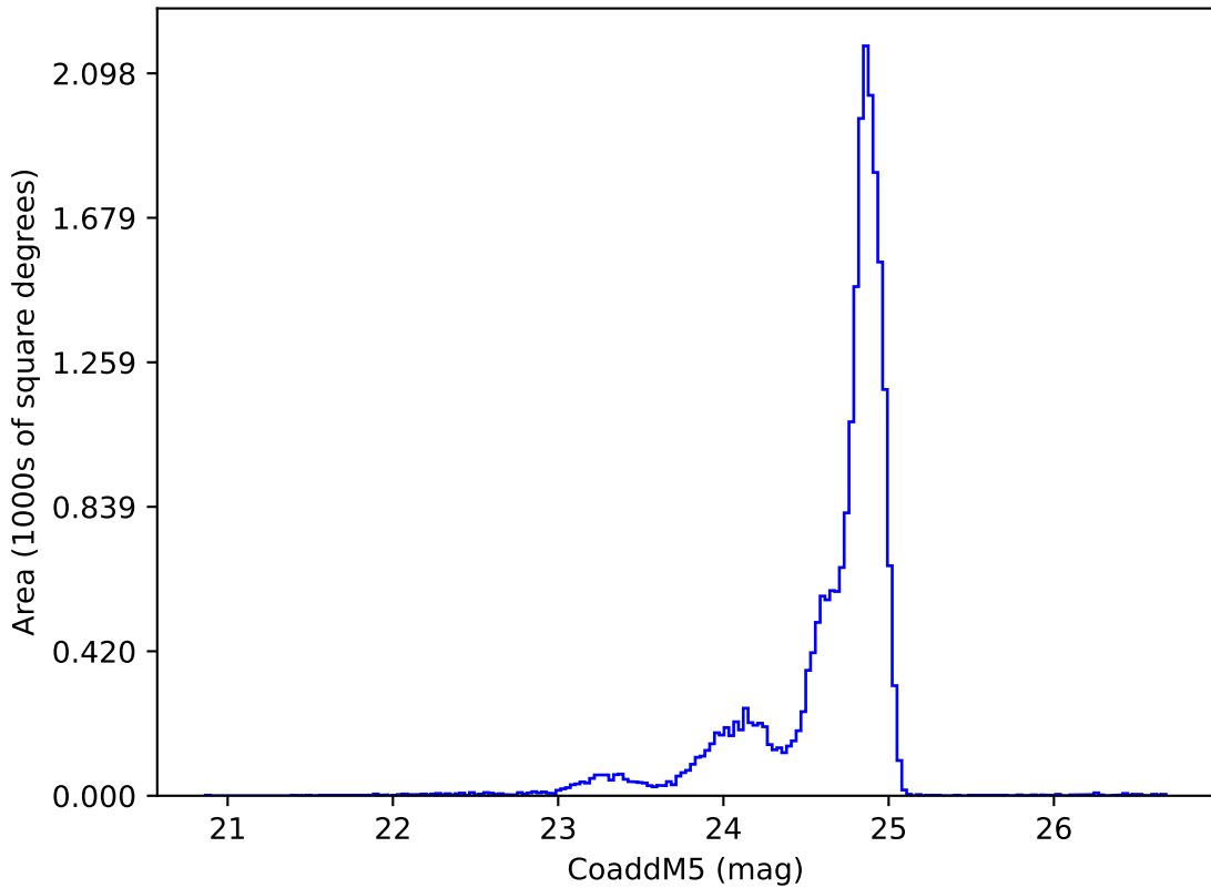
ddf_acor_sf25_lsf40_lsr20_v3.4_10yrs y: CoaddM5
