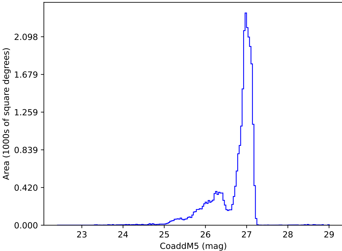
ddf_acor_sf25_lsf40_lsr20_v3.4_10yrs r: CoaddM5
