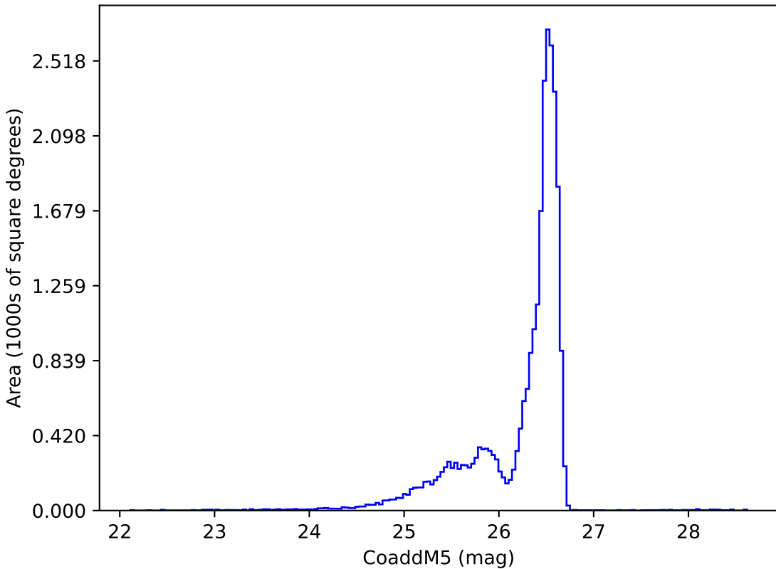
ddf_acor_sf25_lsf40_lsr20_v3.4_10yrs i: CoaddM5
