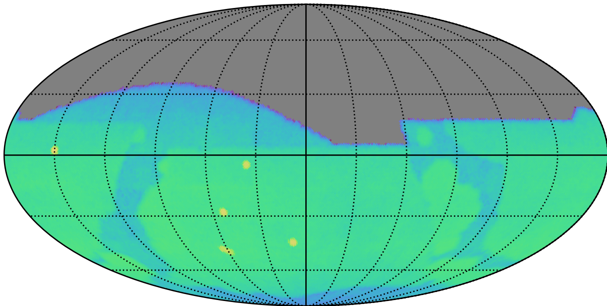
ddf_acor_sf25_lsf40_lsr20_v3.4_10yrs g: CoaddM5
