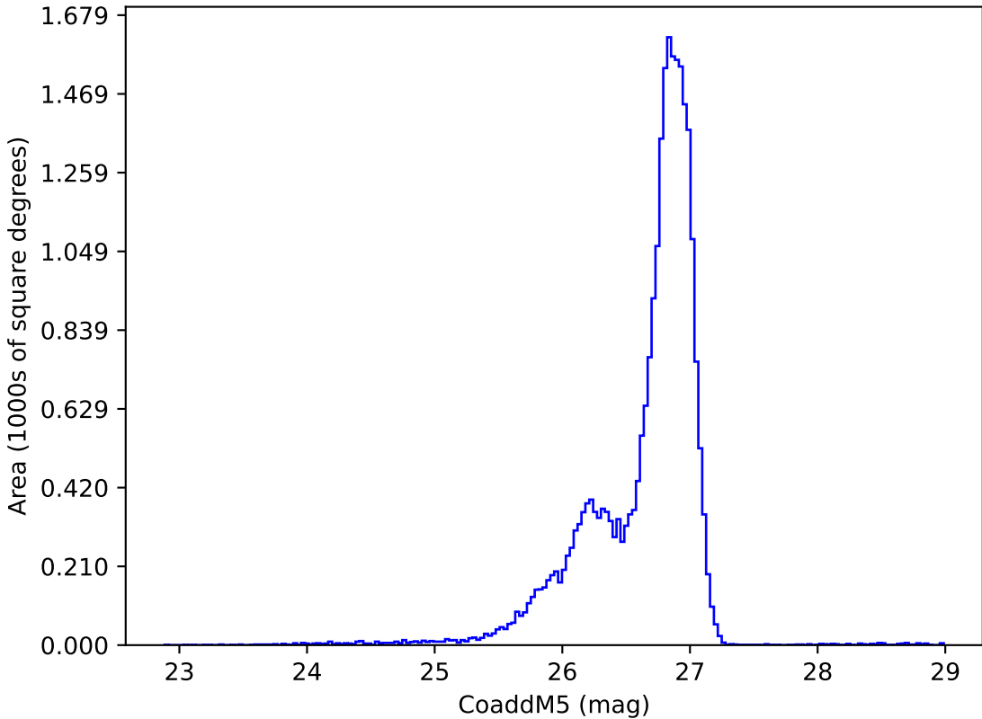
ddf_acor_sf25_lsf40_lsr20_v3.4_10yrs g: CoaddM5
