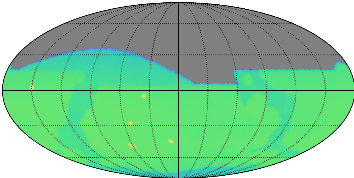
ddf_acor_sf25_lsf40_lsr20_v3.4_10yrs : CoaddM5
