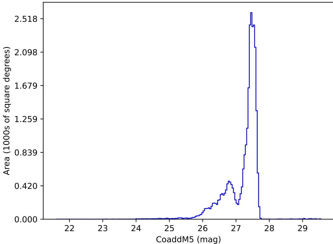
ddf_acor_sf25_lsf40_lsr20_v3.4_10yrs : CoaddM5
