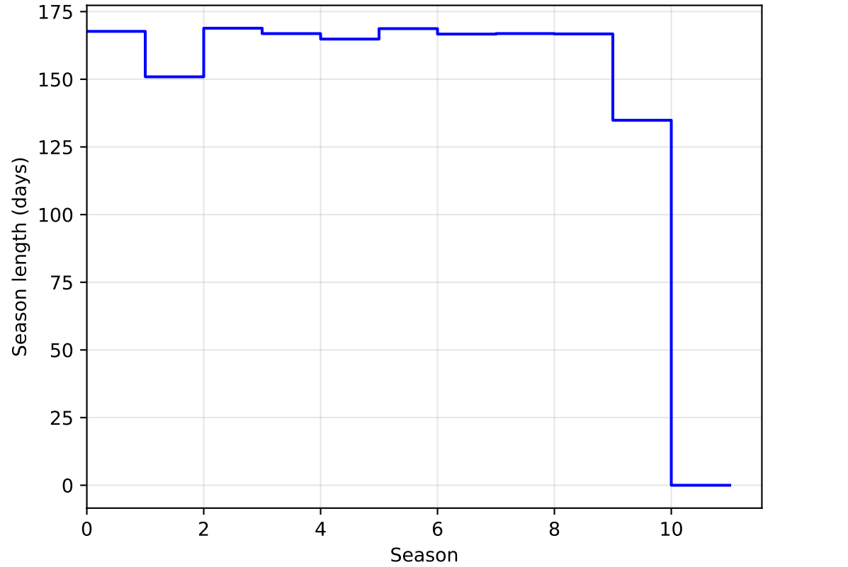
ddf_acor_sf25_lsf40_lsr20_v3.4_10yrs DD:ECDFS all bands: SeasonLength
