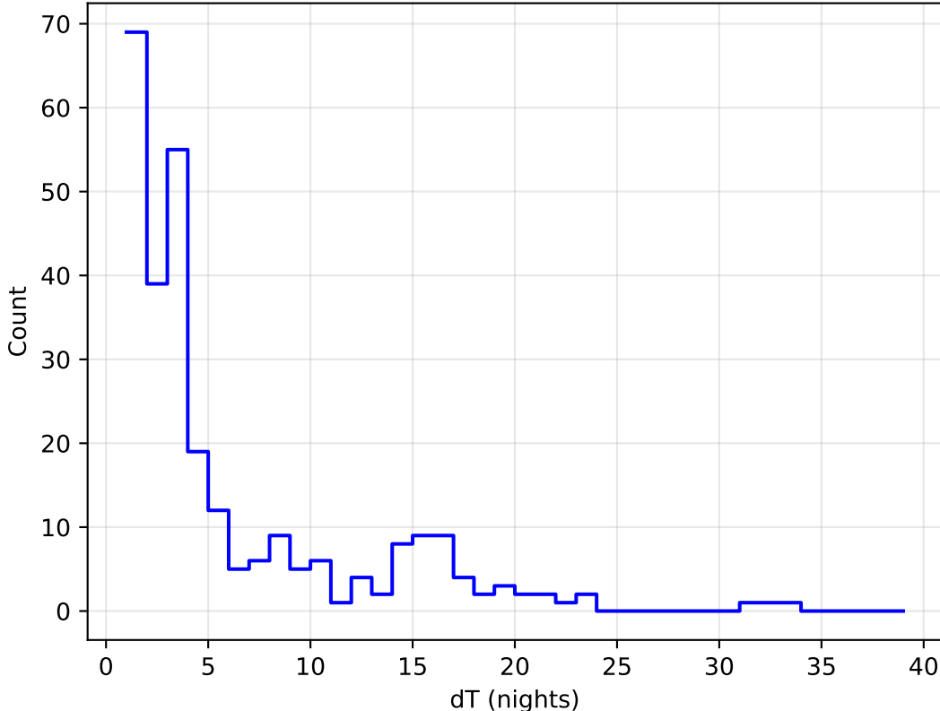
ddf_acor_sf25_Isf40_Isr20_v3.4_10yrs all bands: DD:XMM_LSS Delta Nights Histogram
