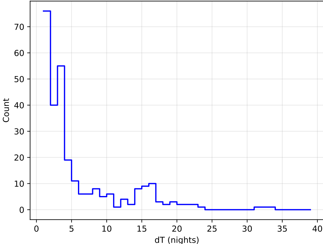
ddf_acor_sf25_lsf40_lsr20_v3.4_10yrs all bands: DD:XMM_LSS Delta Nights Histogram
