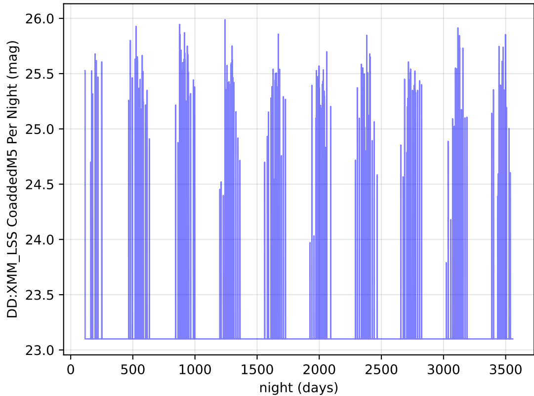
ddf_acor_sf25_lsf40_lsr20_v3.4_10yrs i band: DD:XMM_LSS CoaddedM5 Per Night
