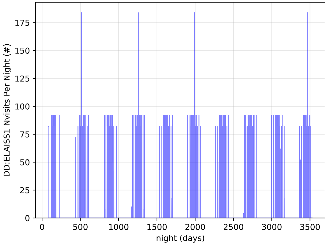
ddf_acor_sf25_lsf40_lsr20_v3.4_10yrs all bands: DD:ELAISS1 Nvisits Per Night
